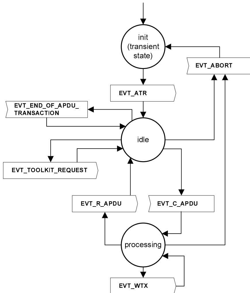
Figure 10.2: State transitions
